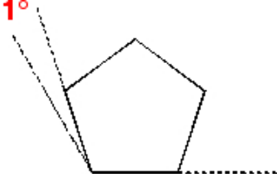
cyclopentane
