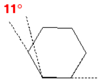
cyclohexane
