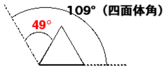
cyclopropane
